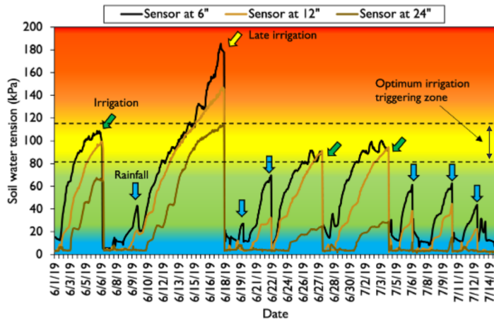
Figure 3. Dynamic soil water tension values over the period of peak water demand for corn (R1 to R5) at soil depths of 6, 12, and 24 inches for a cornfield cultivated on a silty clay loam soil in northwestern Alabama. Irrigation is represented by green arrows and rainfall by blue arrows.
