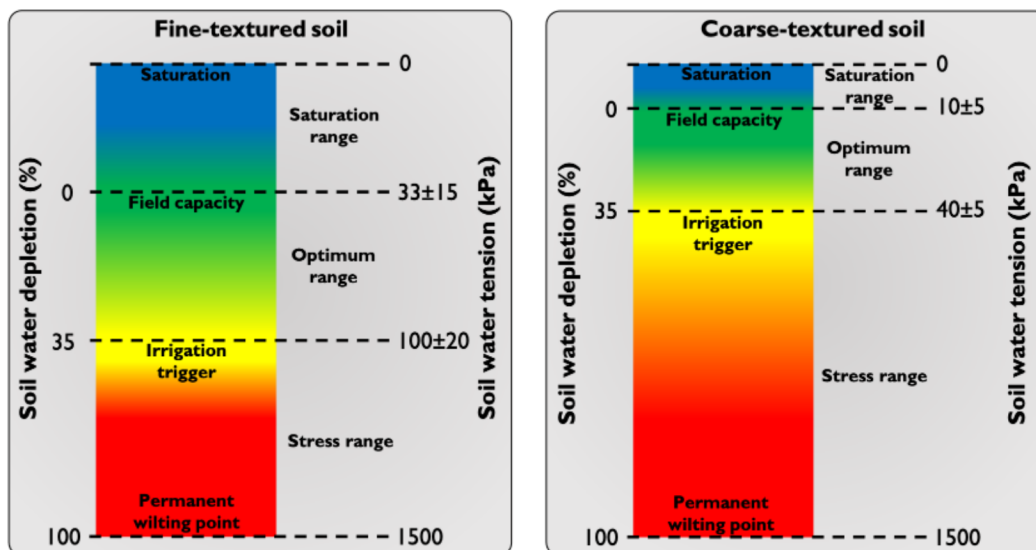
Figure 2. Relationship between soil water tension and soil water depletion and the different water levels used for irrigation purposes in fine-textured soil (left) and coarse-textured soil (right).
