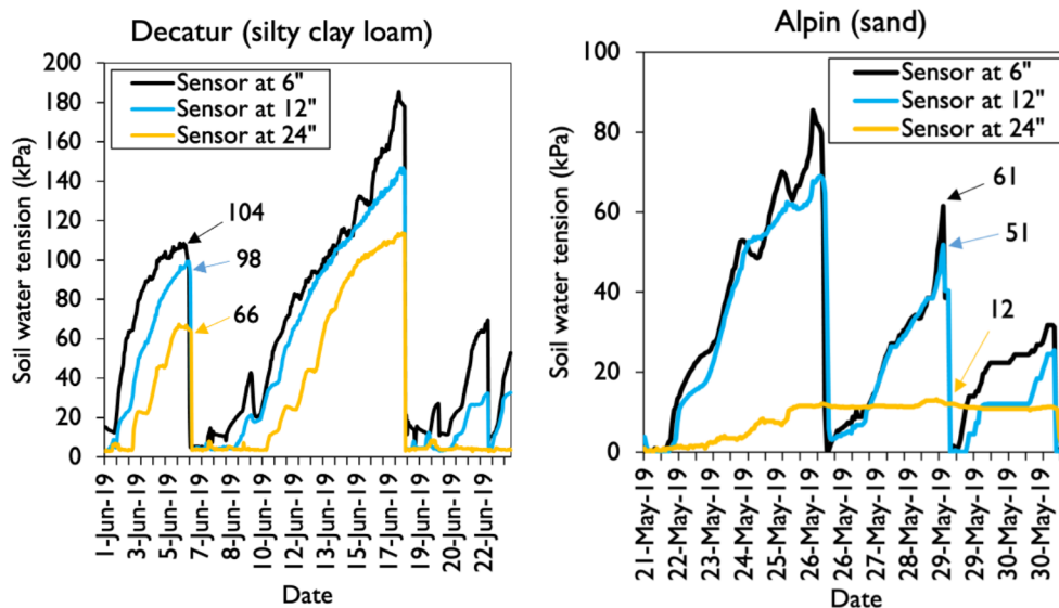
Figure 4. Dynamics of soil water tension values at soil depths of 6, 12, and 24 inches at two cornfields cultivated on a silty clay loam (left) and a sand soil (right). Black, blue, and orange arrows represent the soil water tension value for the soil sensor at 6, 12, and 24 inches, respectively.
